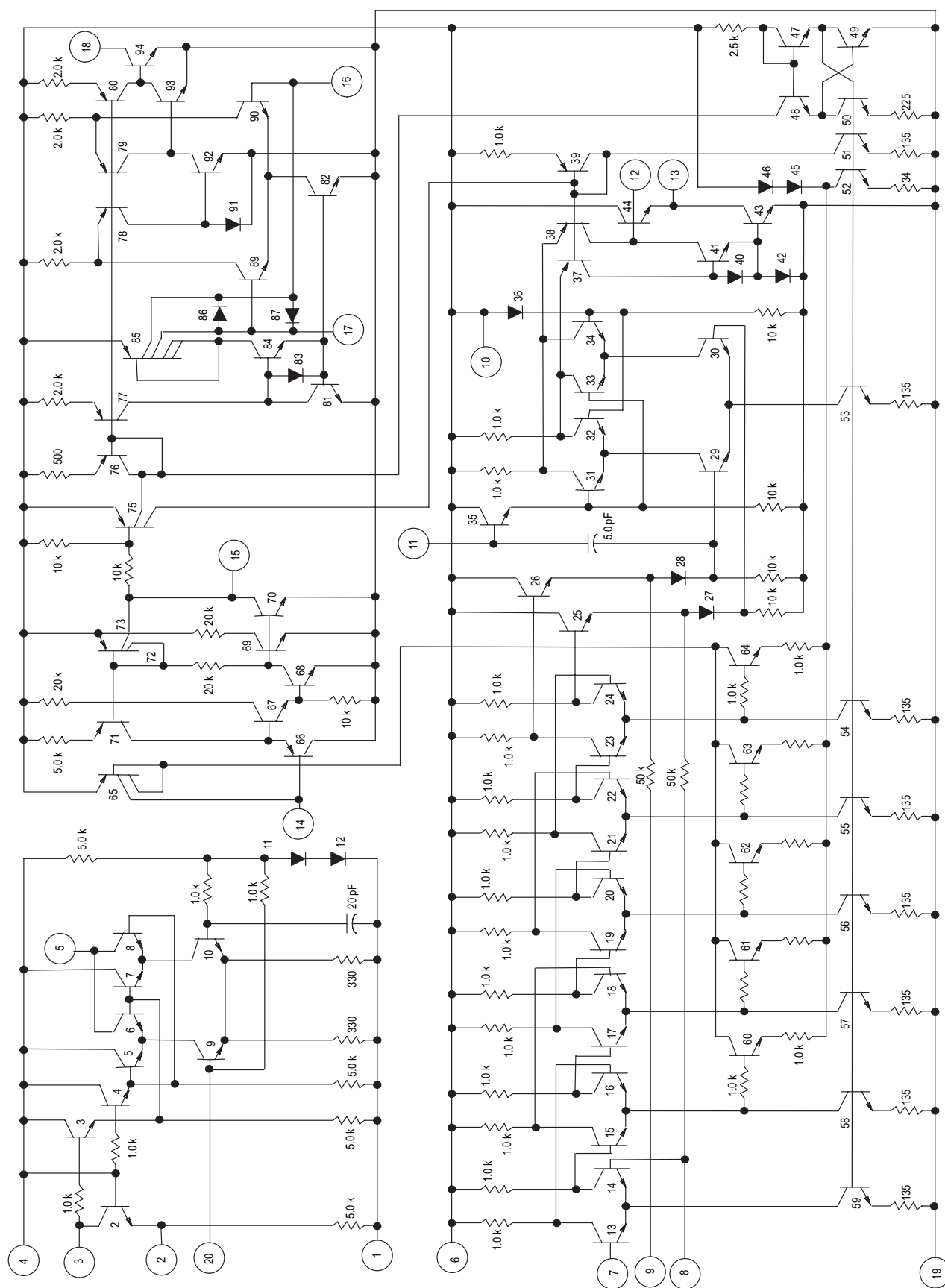
Figure 7. Internal Schematic
