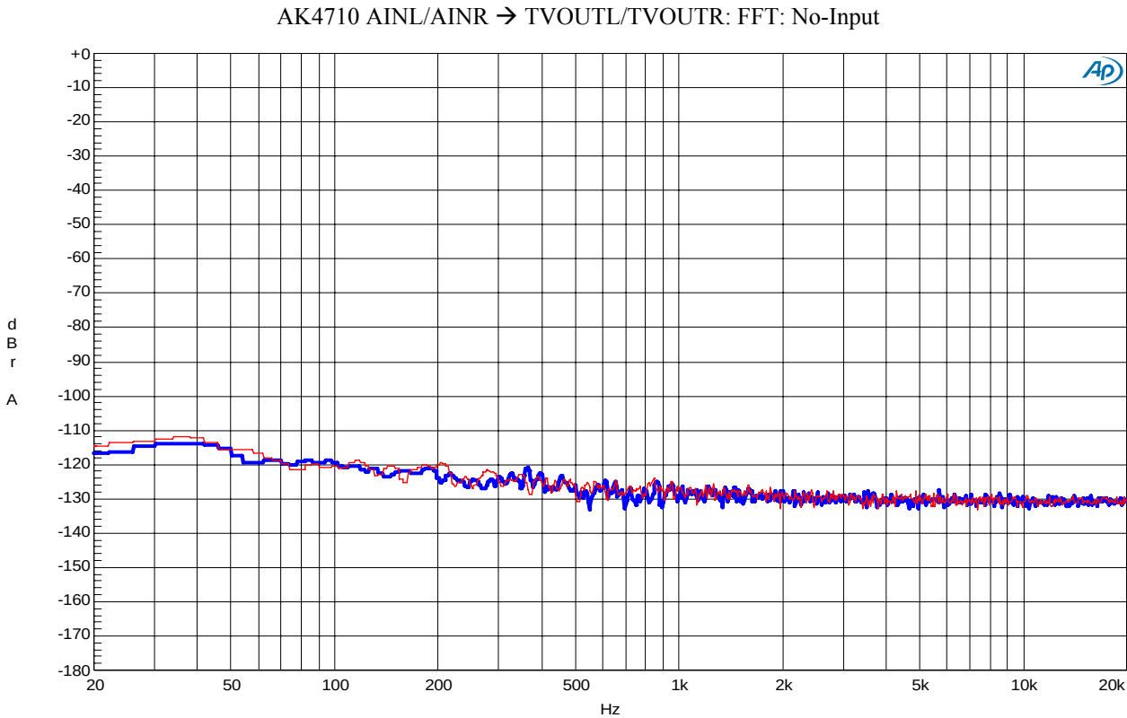
Figure1-3. FFT (Noise Floor)
