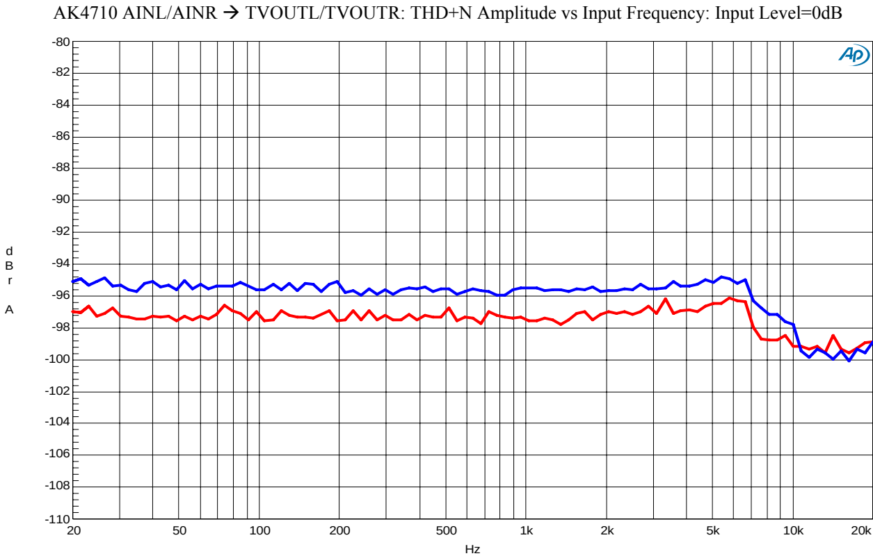
Figure1-5. THD+N vs. Input Frequency (Input level=0dB)
