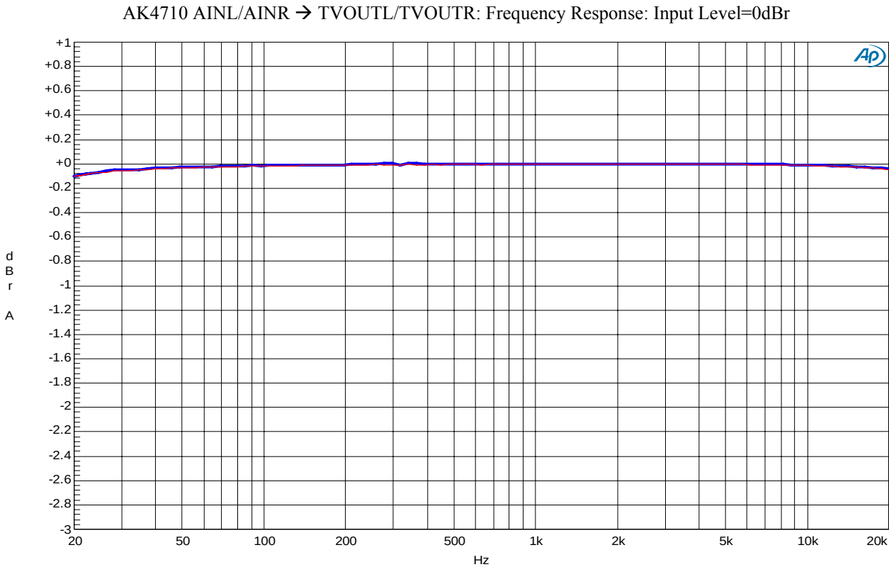
Figure1-7. Frequency Response (Input level=0dB)
