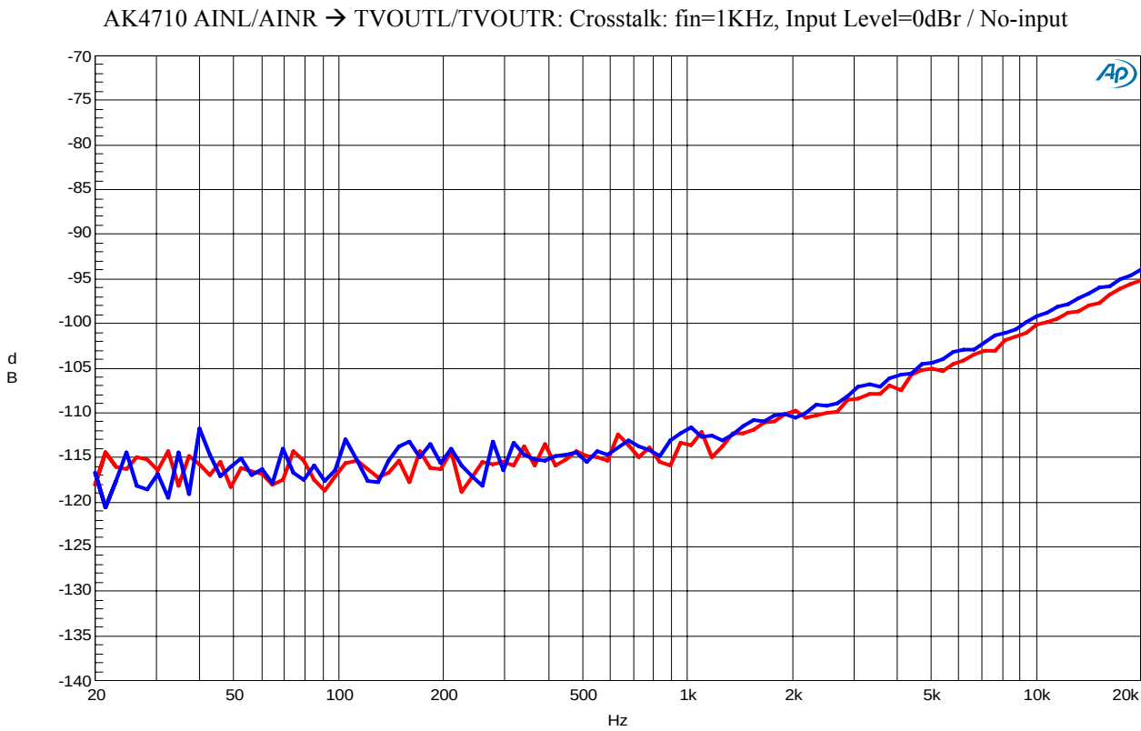
Figure1-8. Crosstalk (Input level=0dB)
