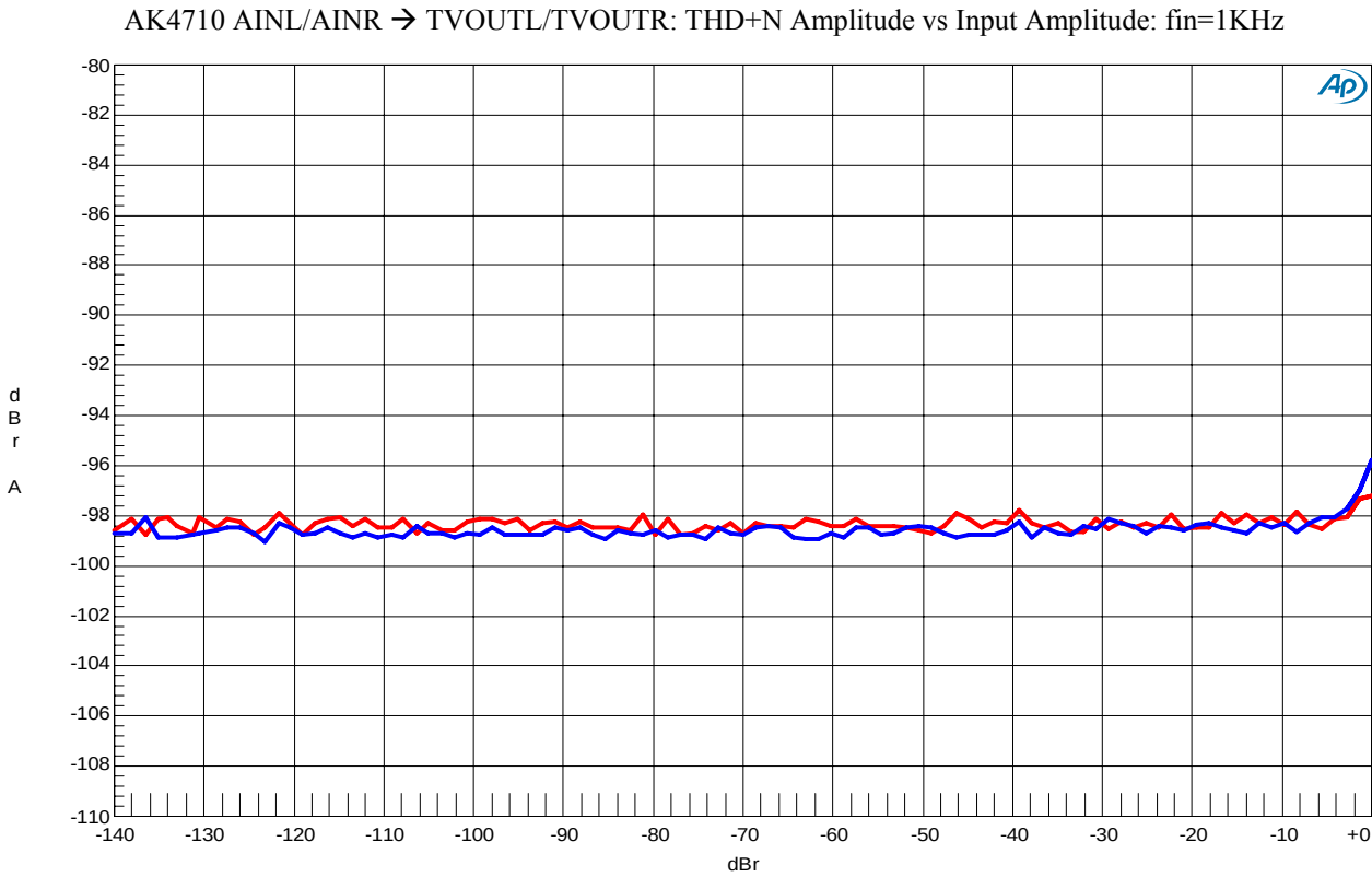
Figure1-4. THD+N vs. Input level (fin=1kHz)
