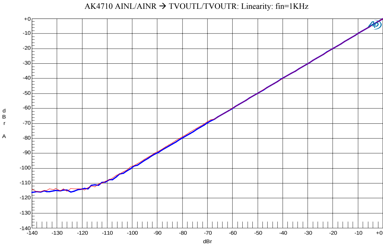
Figure1-6.Linearity (fin=1kHz)
