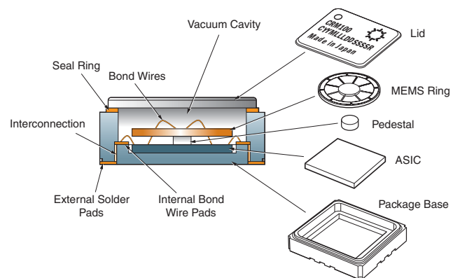
Figure 13.1 CRM100 Main Components
