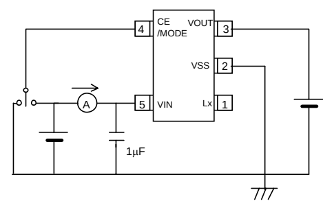
Circuit ③
