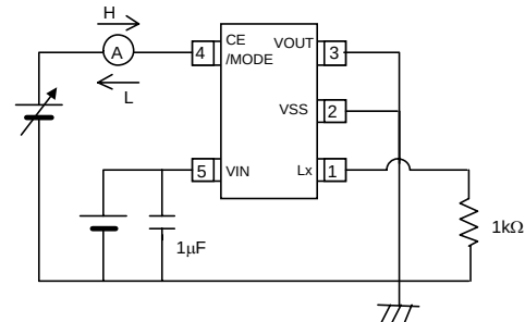
Circuit ⑤
