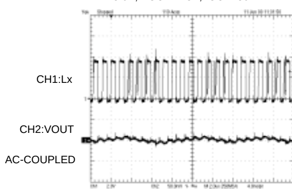
③ VIN=3.6V, VOUT=1.8V, IOUT=30mA
