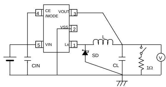
Circuit ⑥
