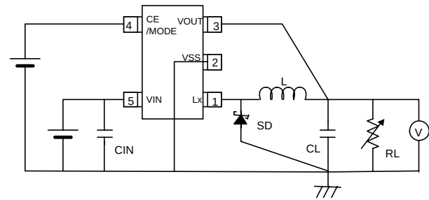
Circuit ①
