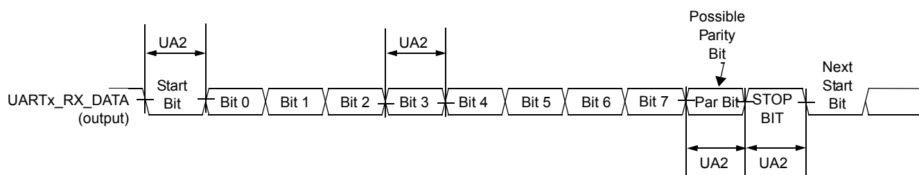
Figure 64. UART RS-232 Serial Mode Receive Timing Diagram
