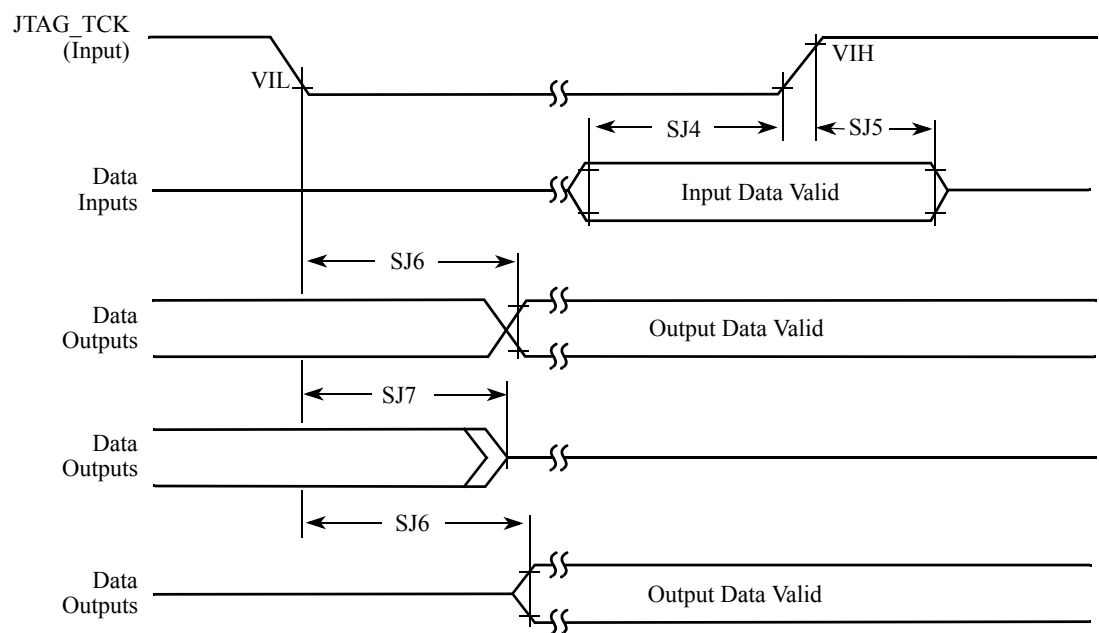
Figure 58. Boundary Scan (JTAG) Timing Diagram
