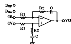
Differential filter
