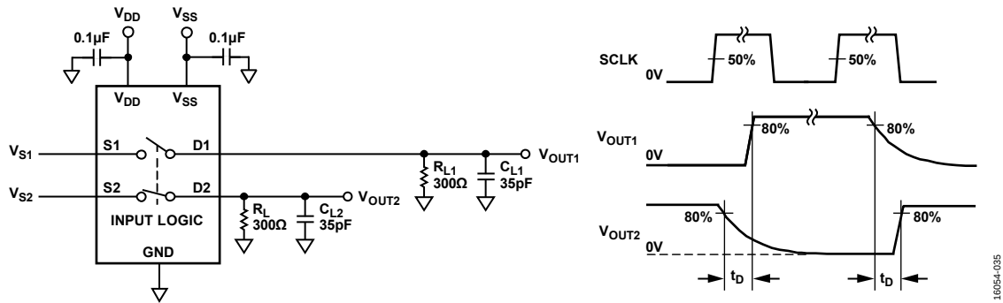
Figure 35. Break-Before-Make Time Delay, t_D
