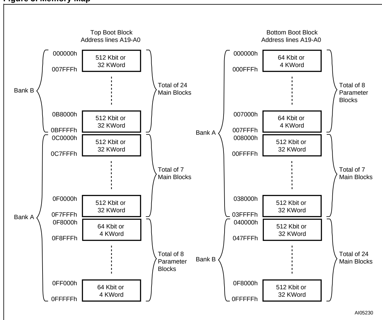
Figure 3. Memory Map
