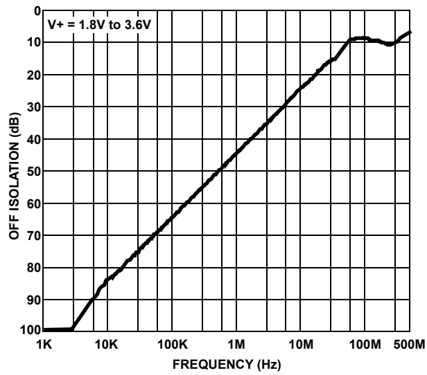
FIGURE 15. OFF ISOLATION
