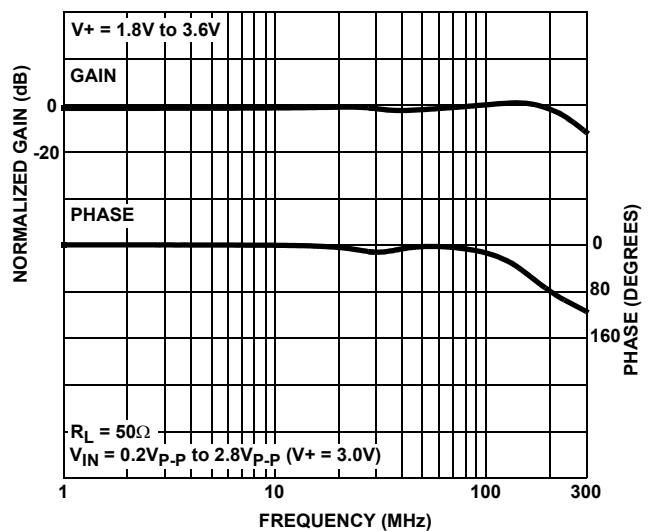
FIGURE 14. FREQUENCY RESPONSE
