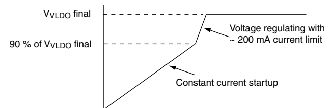
Figure 9 - LDO Start-Up
