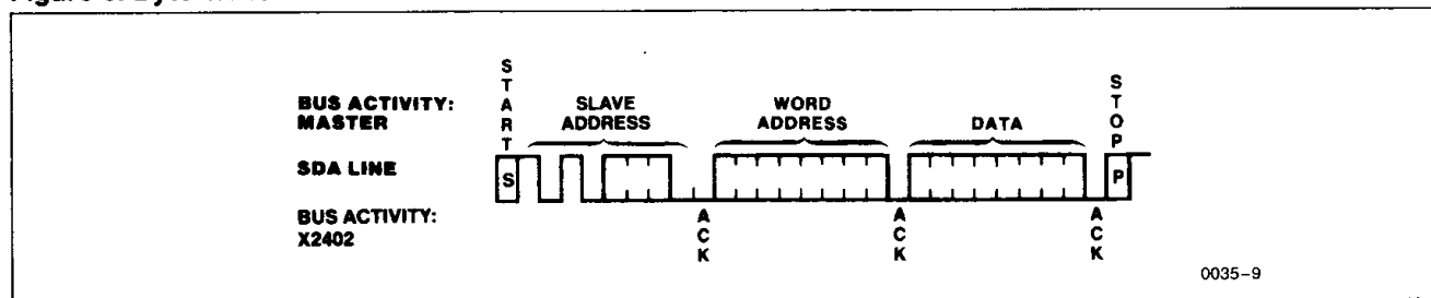
Figure 5: Byte Write
