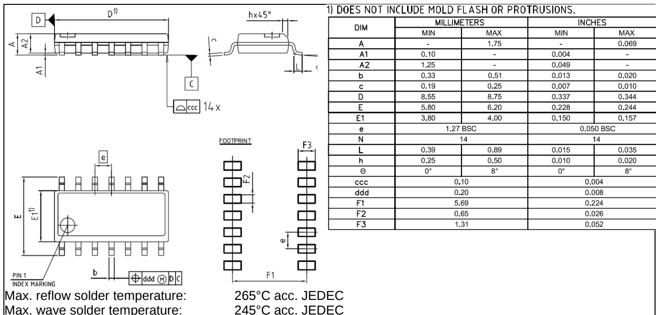
Figure 14 Package drawing
