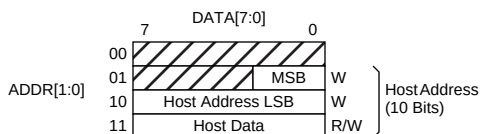
Figure 16. Address Space of ZR36060 in Code Master Mode
