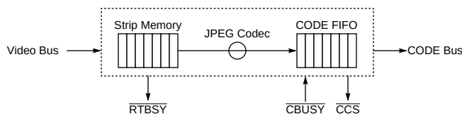
Figure 30. Data Flow in Compression, Code Master
