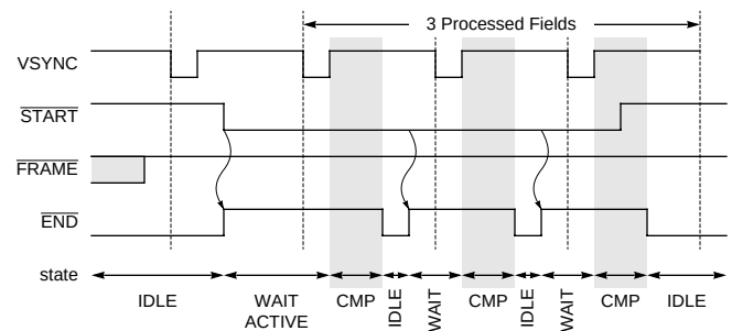
Figure 35. Compression with continuous \overline{\text{START}} asserted and \overline{\text{FRAME}} Deasserted
