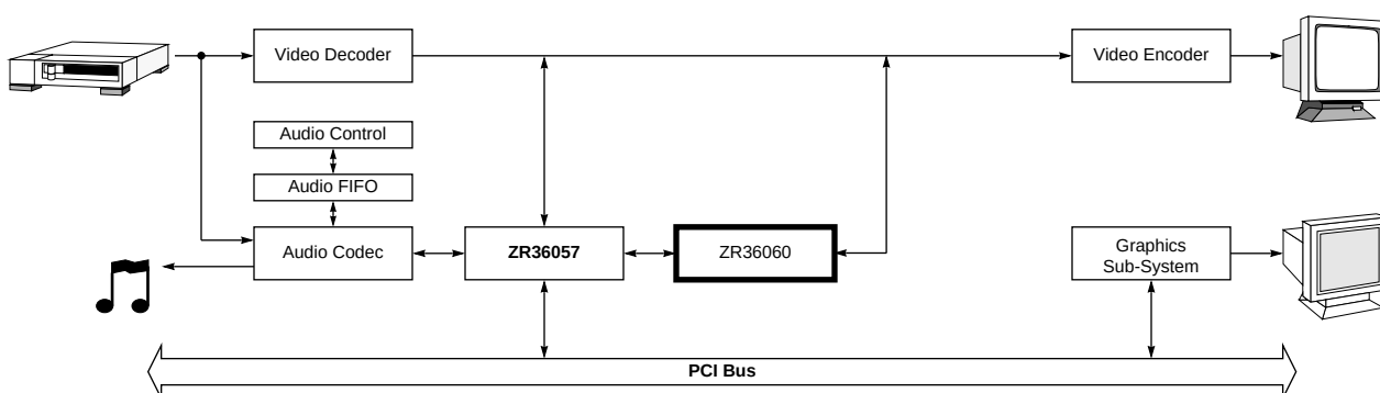
Figure 1. JPEG-based video editing subsystem for PCI Systems
