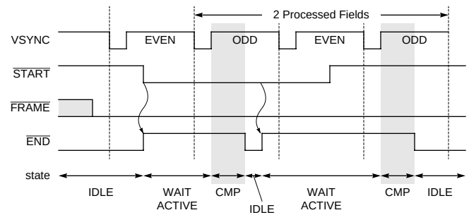
Figure 34. Compression with \overline{\text{START}} and \overline{\text{FRAME}} continuously asserted
