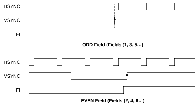
Figure 4. Field Detection Showing Hor. and Ver. Timing
