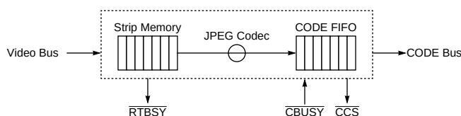
Figure 31. Data Flow in Compression, Code Master
