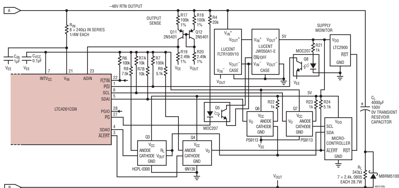
Figure 2b. 200W AdvancedTCA Hot Swap Controller with Input/Output Monitoring and Power Good Watchdog Using LTC4261 in I²C Mode (Part Two)
