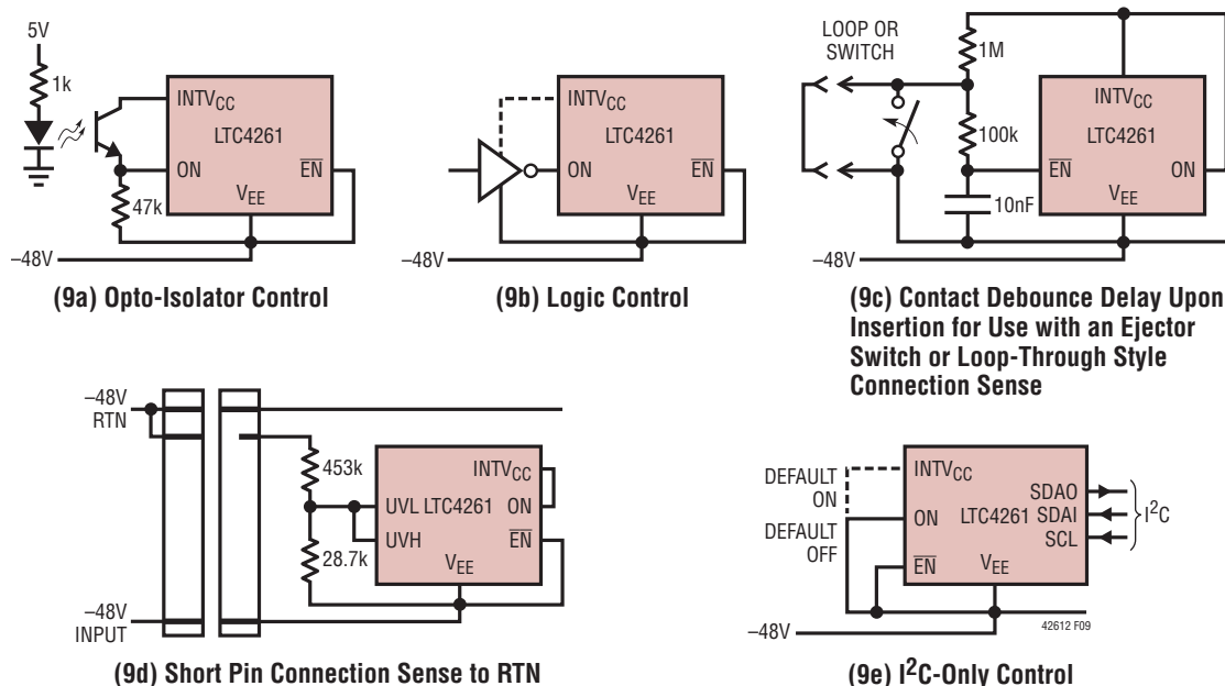
Figure 9. On/Off Control of the LTC4261
