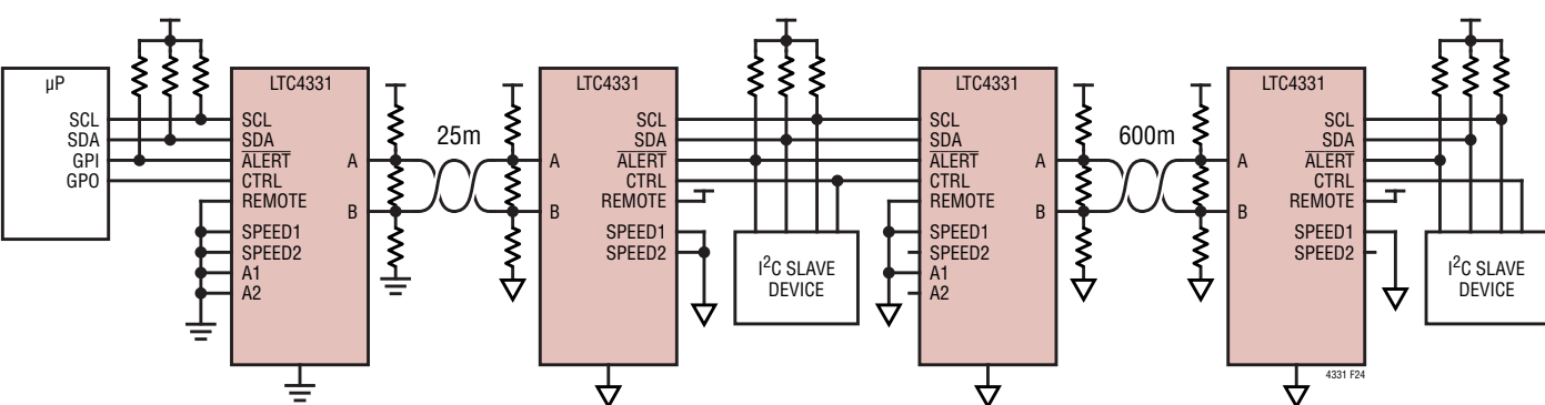
Figure 24. Multi-Tier Extender Network
