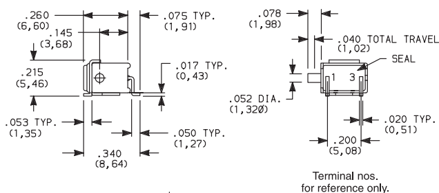
PC MOUNTING
