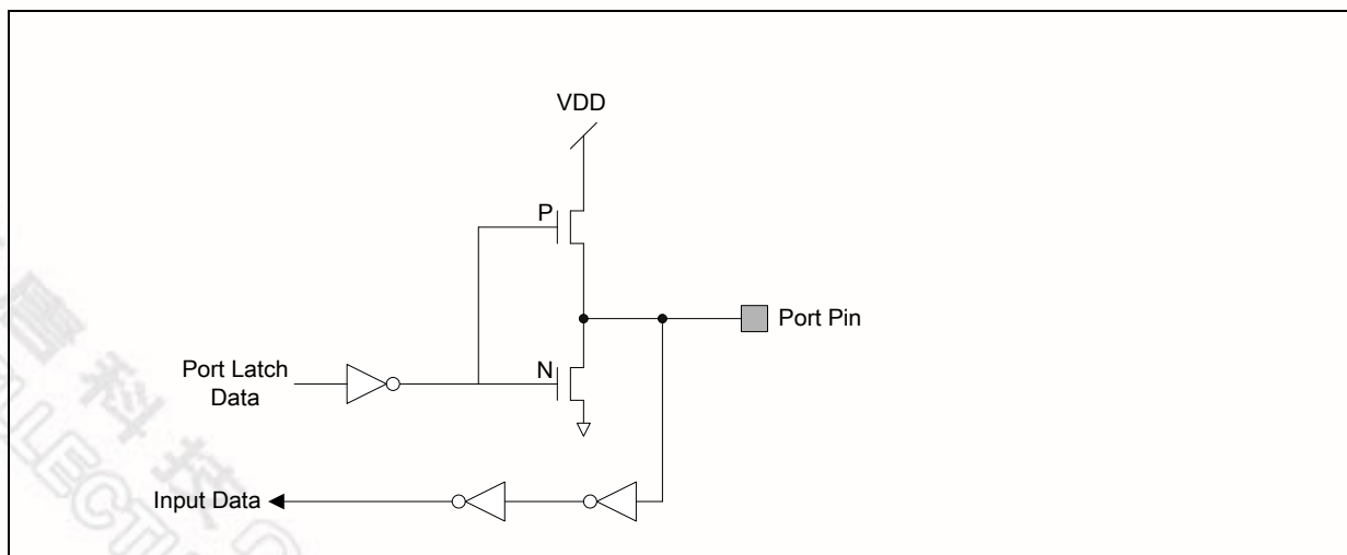
Figure 22-3: Push-Pull Output
