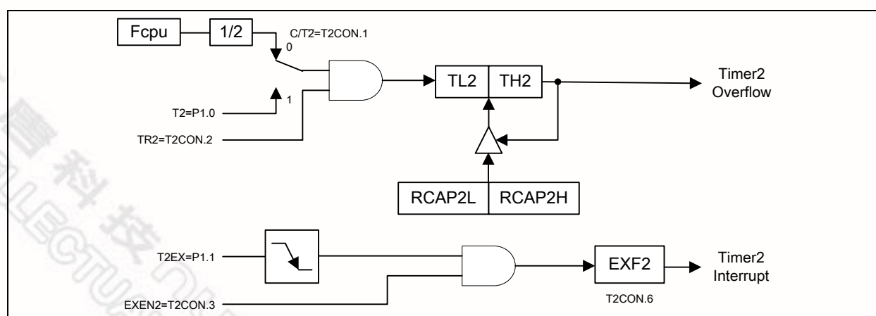
Figure 12-7: Baud Rate Generator Mode
