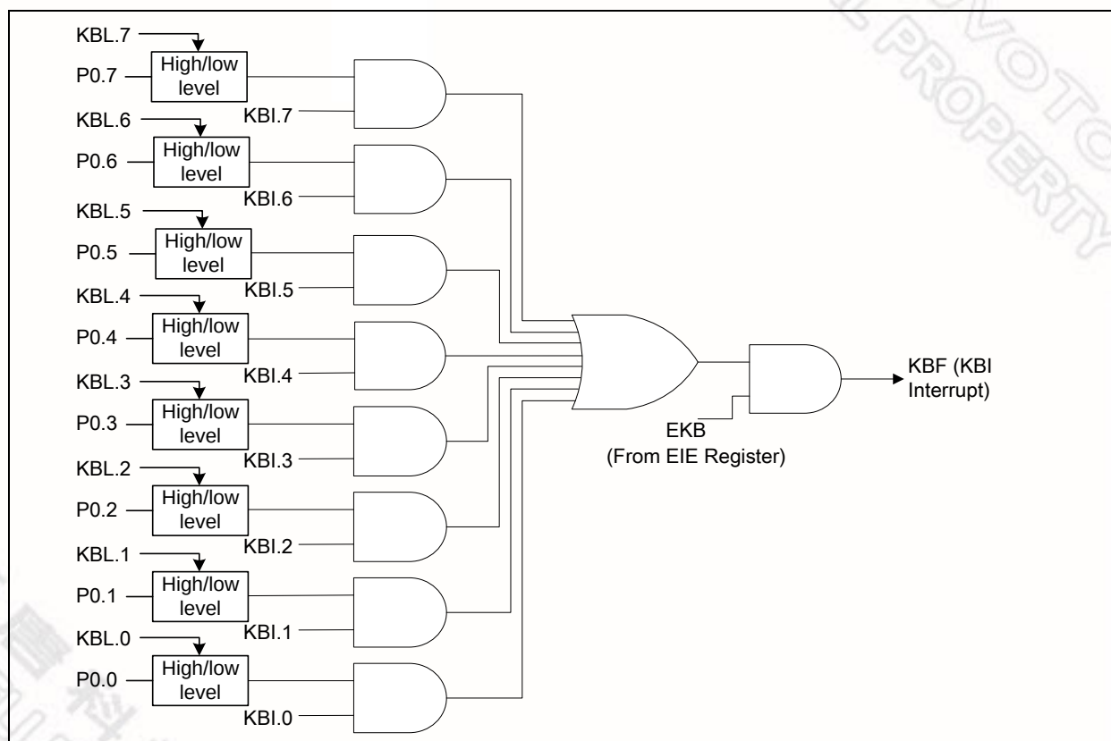
Figure 19-1: KBI inputs
