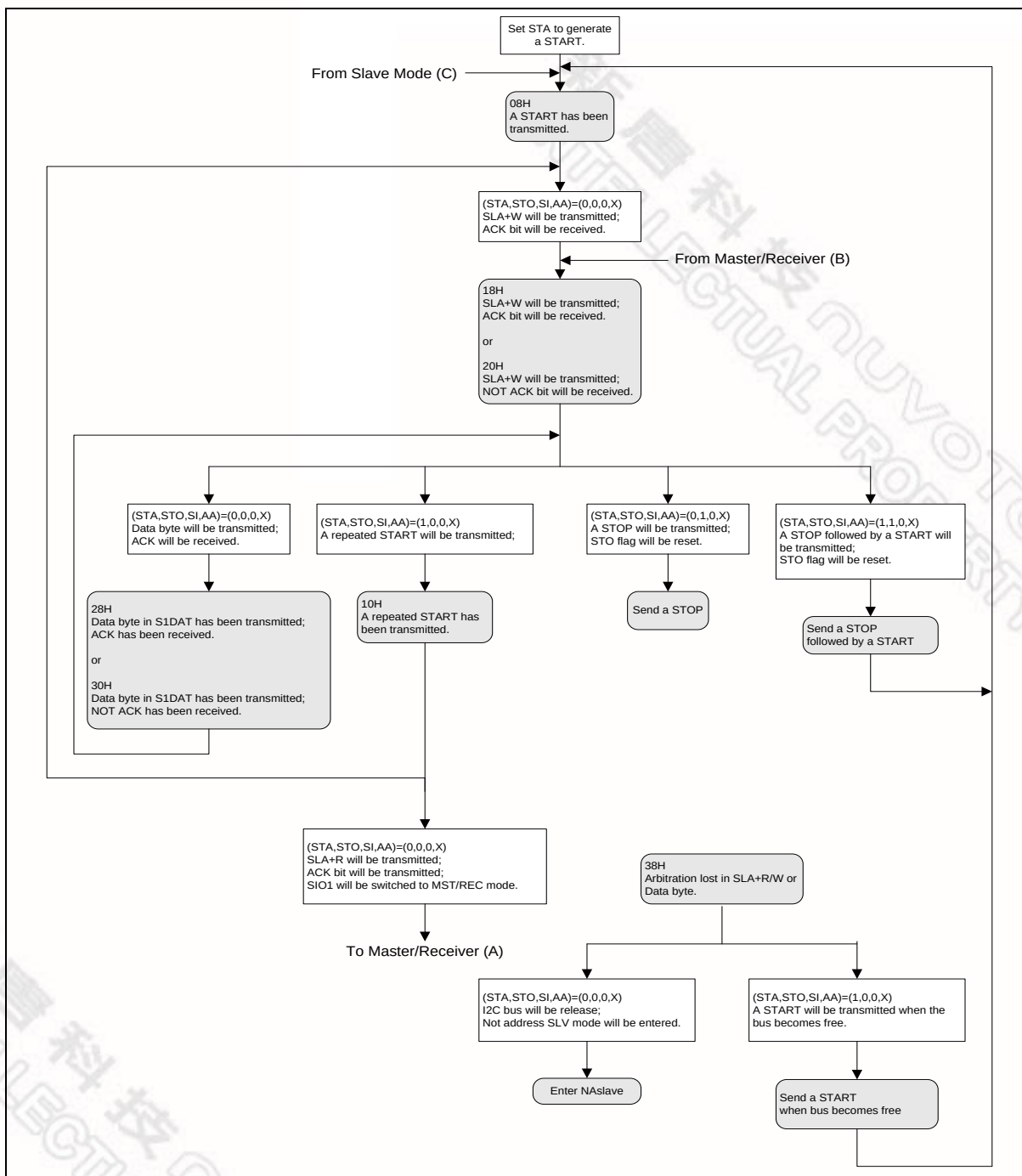
Figure 16-4: Master Transmitter Mode
