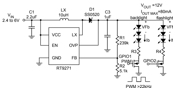
Figure 9. Constant output voltage for backlight and flashlight
