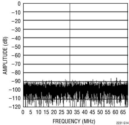
LTC2231: 8192 Point FFT, f_{IN} = 30\text{MHz} , -1dB, 2V Range
