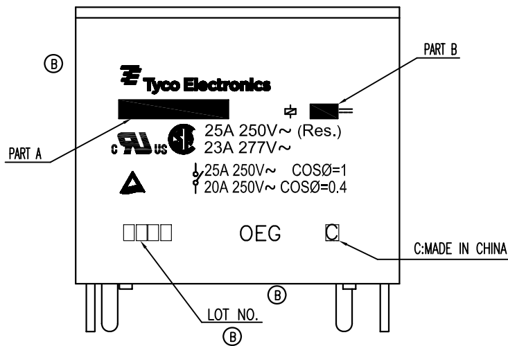
VIEW C
