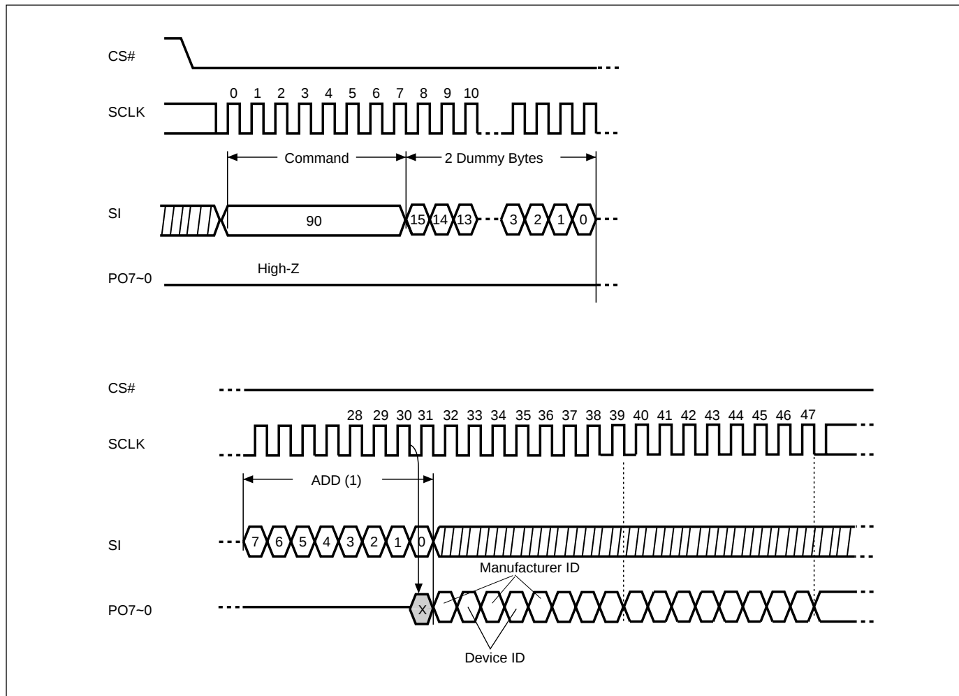
Figure 34. Read Electronic Manufacturer & Device ID (REMS) Sequence (Parallel)
