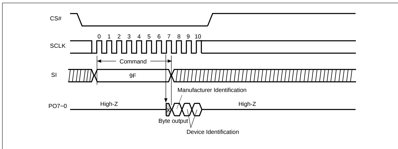
Figure 31. Read Identification (RDID) Sequence (Parallel)
