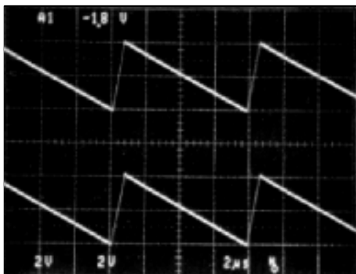
Graph 17. 128kHz Sawtooth Waveform Response
