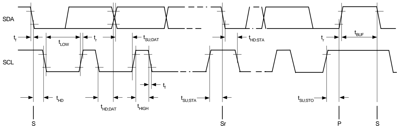
Figure 7. I 2 C Timing Diagram
