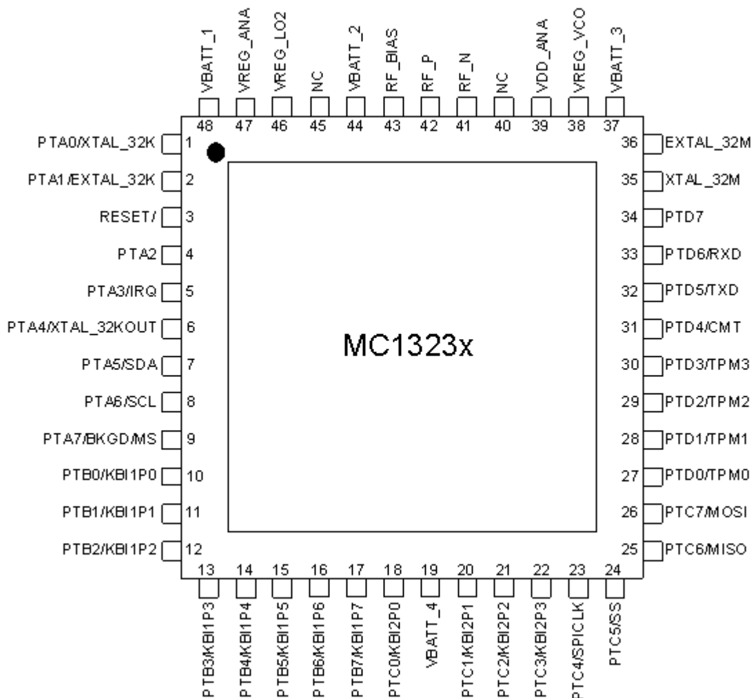
Figure 2. MC1323x Pinout
