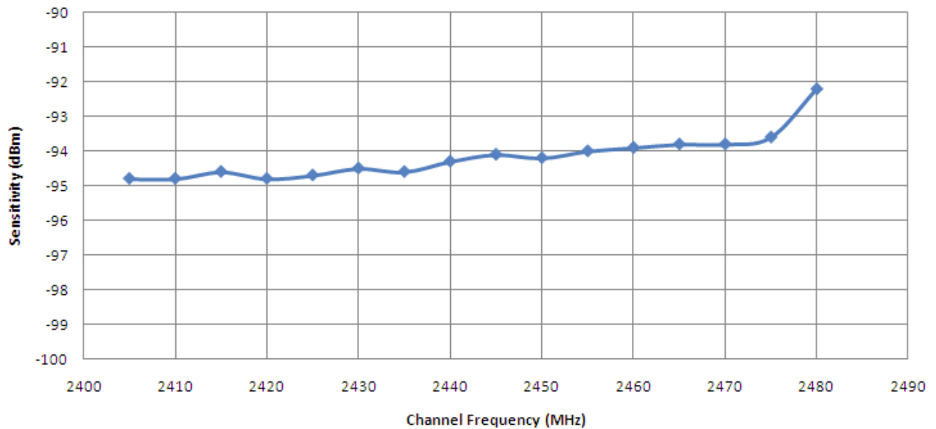
Figure 3. Typical RX Sensitivity vs. Channel Frequency @ 25°C
