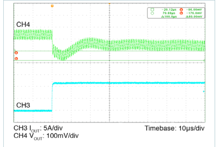
Figure 14 — Load transient response, nominal line Load step 0-25%
