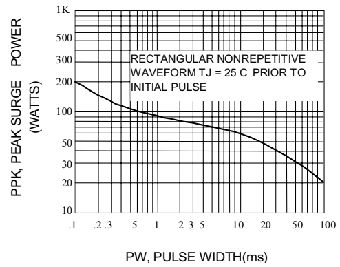
Fig. 4- PULSE RATING CURVE
