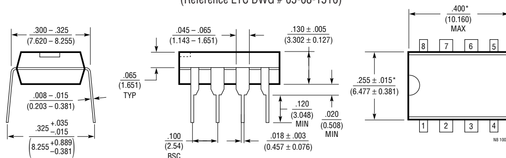
N8 Package 8-Lead PDIP (Narrow .300 Inch) (Reference LTC DWG # 05-08-1510)
