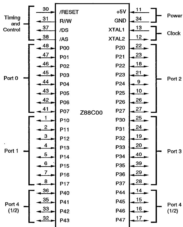
Figure 5. Pin Functions
