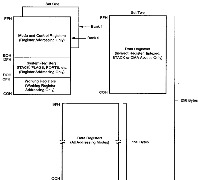
Figure 6. Super8 Registers
