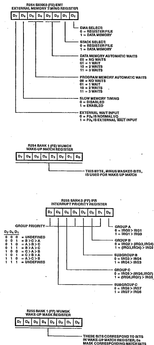
Figure 8. Mode and Control Registers (Continued)
