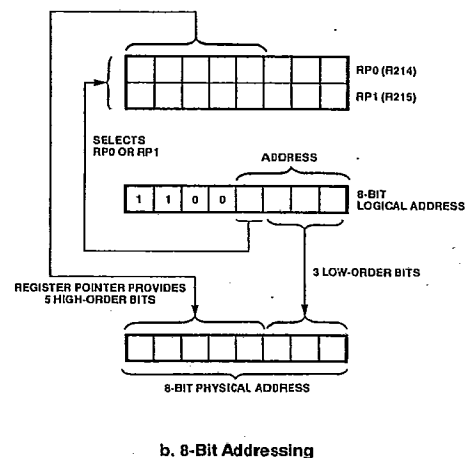
Figure 7. Working Register Window
