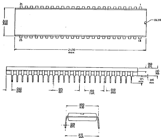
48-Lead DIP Package
