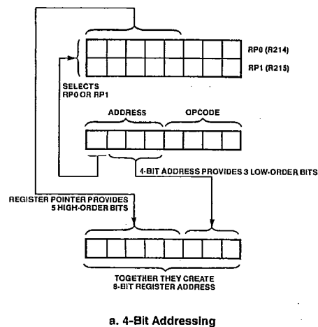
Figure 7. Working Register Window
