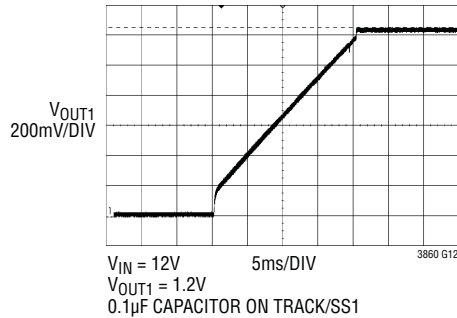
Soft-Start Start-Up
