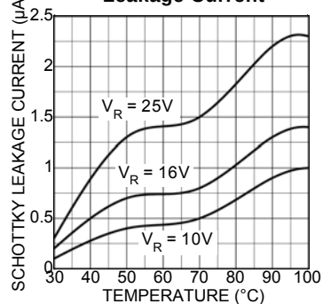
Schottky Reverse Leakage Current
