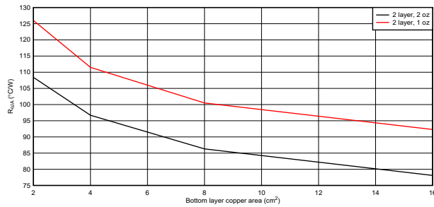
Figure 10-13. WQFN, PCB junction-to-ambient thermal resistance vs copper area
