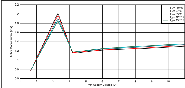
Figure 8-1. Active Mode Current
