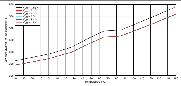
Figure 8-4. Low-side MOSFET on resistance
