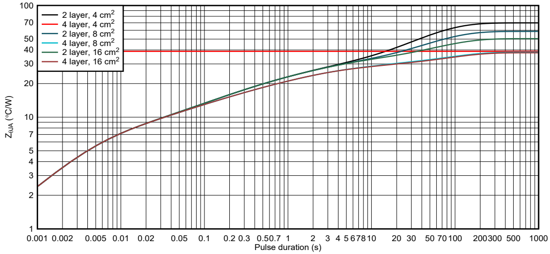
Figure 10-15. HTSSOP package junction-to-ambient thermal impedance for 1-oz copper layouts
