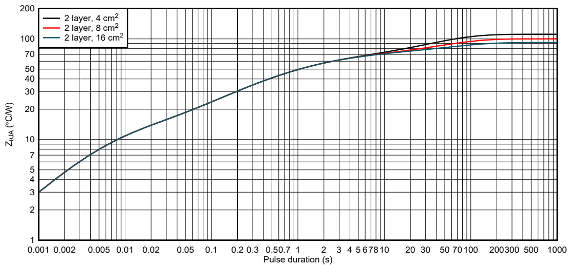
Figure 10-17. WQFN package junction-to-ambient thermal impedance for 1-oz copper layouts
