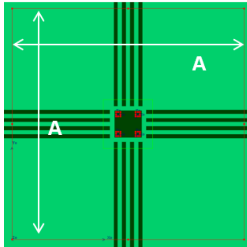
Figure 10-10. WQFN PCB model top layer
