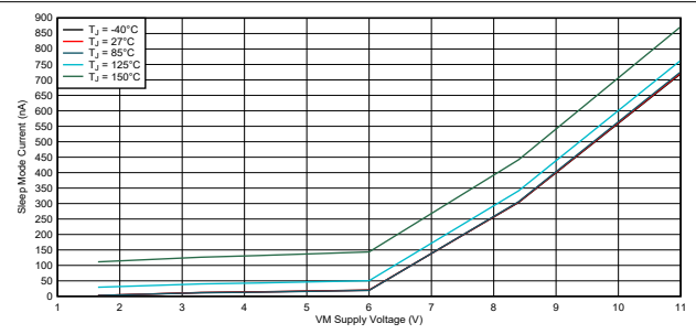
Figure 8-2. Sleep Mode Current
