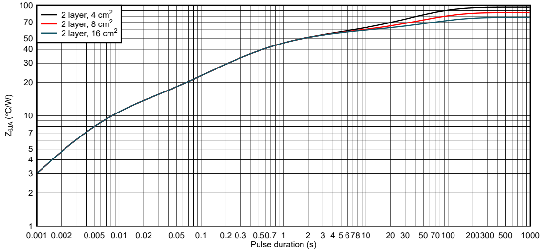
Figure 10-18. WQFN package junction-to-ambient thermal impedance for 2-oz copper layouts
