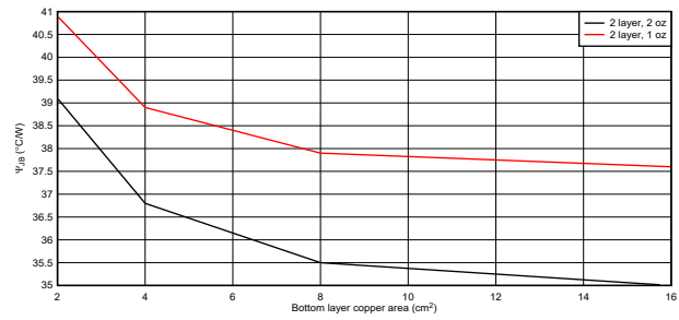
Figure 10-14. WQFN, junction-to-board characterization parameter vs copper area
