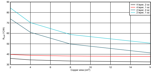
Figure 10-11. HTSSOP, PCB junction-to-ambient thermal resistance vs copper area
