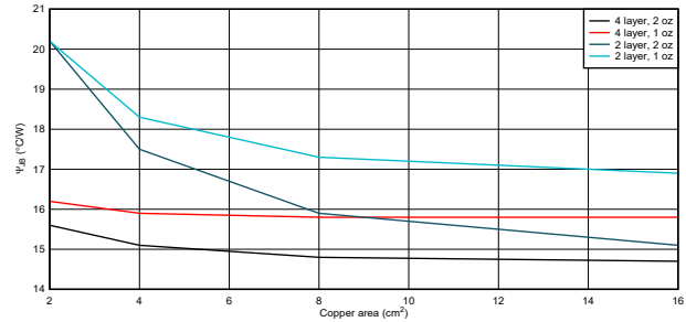
Figure 10-12. HTSSOP, junction-to-board characterization parameter vs copper area
