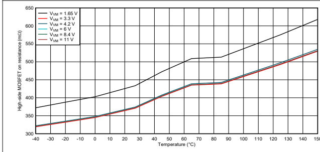
Figure 8-3. High-side MOSFET on resistance
