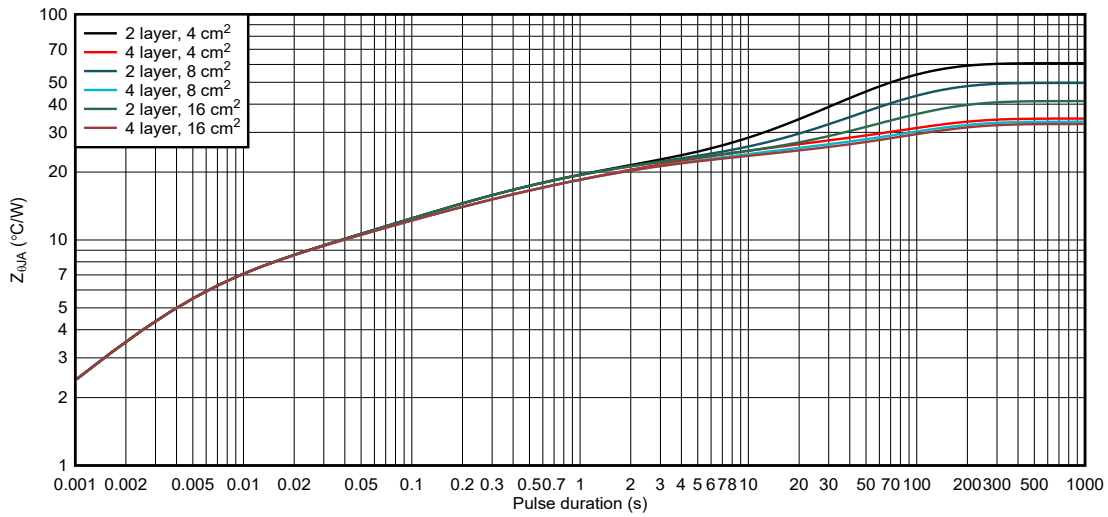
Figure 10-16. HTSSOP package junction-to-ambient thermal impedance for 2-oz copper layouts
