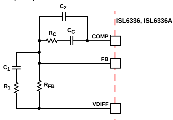
FIGURE 20. COMPENSATION CIRCUIT FOR ISL6336, ISL6336A BASED CONVERTER WITHOUT LOAD-LINE REGULATION
