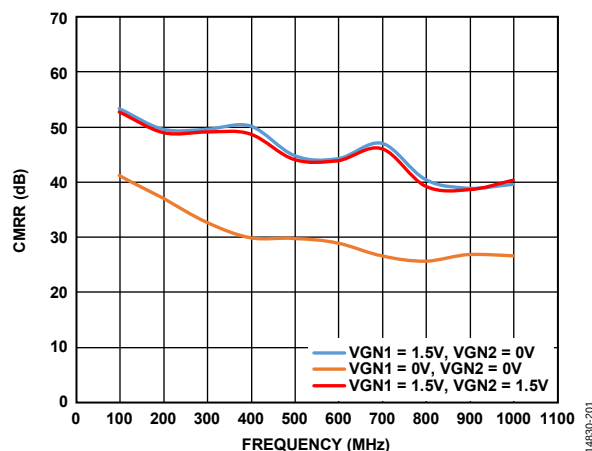
Figure 61. Common-Mode Rejection Ratio (CMRR) vs. Frequency, Bypass Mode
