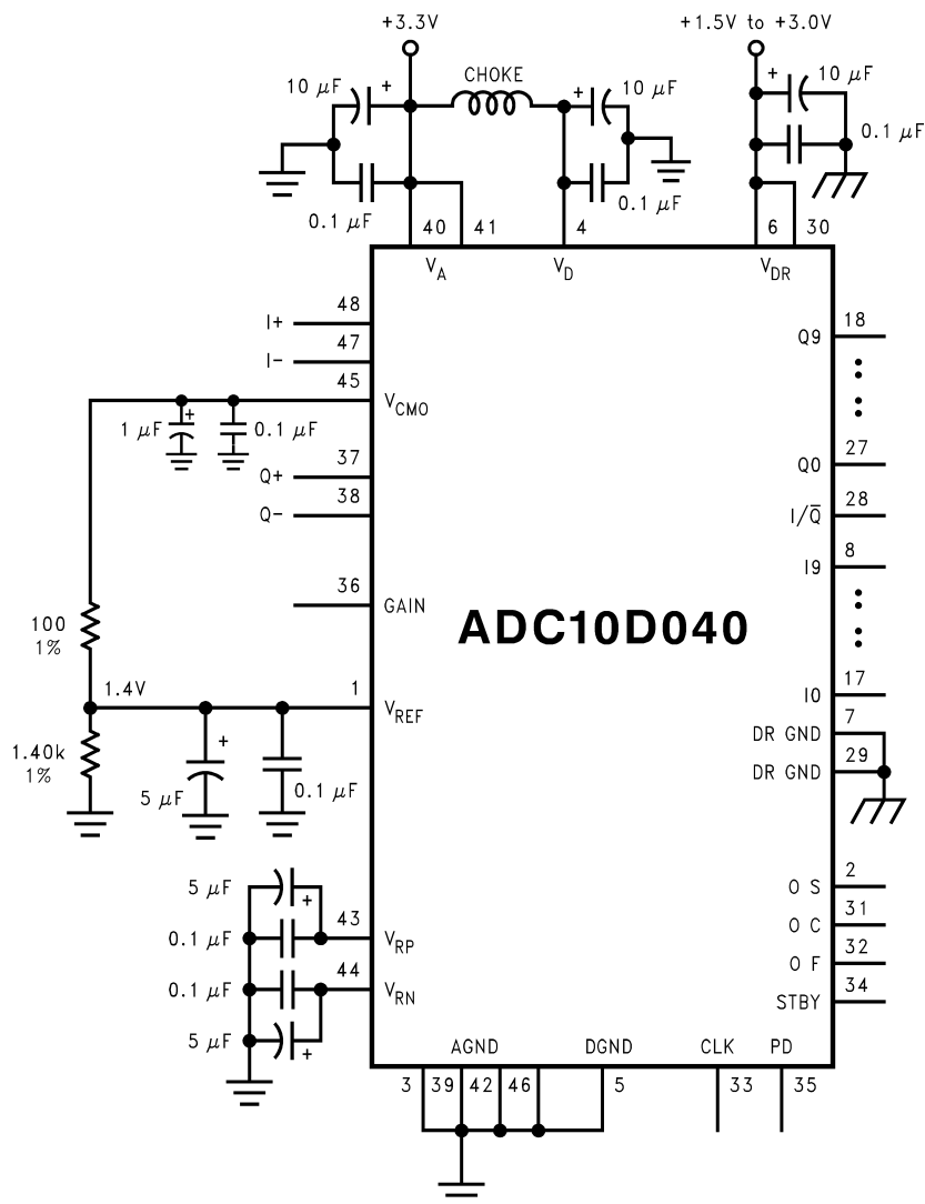
FIGURE 7. The V_{CMO} output pin may be used as an internal reference source if its output is not loaded excessively.
