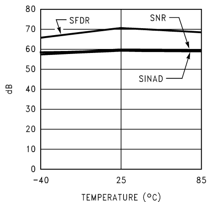
SNR, SINAD & SFDR vs. Temperature
