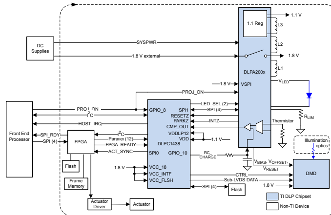
Figure 8-3. Internal Pattern Streaming Mode
