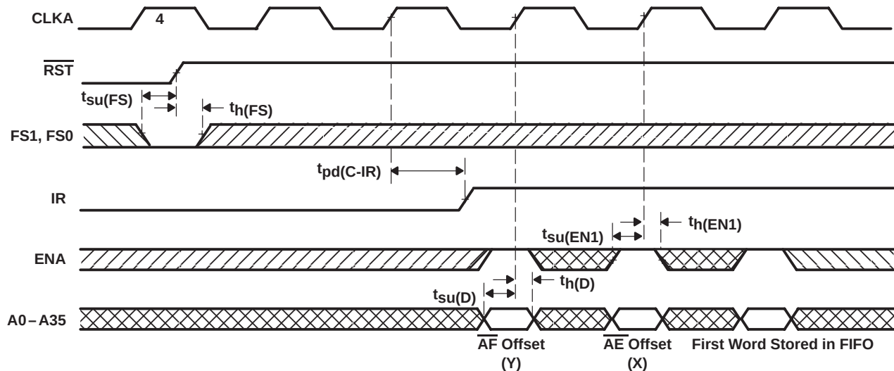
Figure 2. Programming the \overline{\text{AF}} Flag and \overline{\text{AE}} Flag Offset Values From Port A
