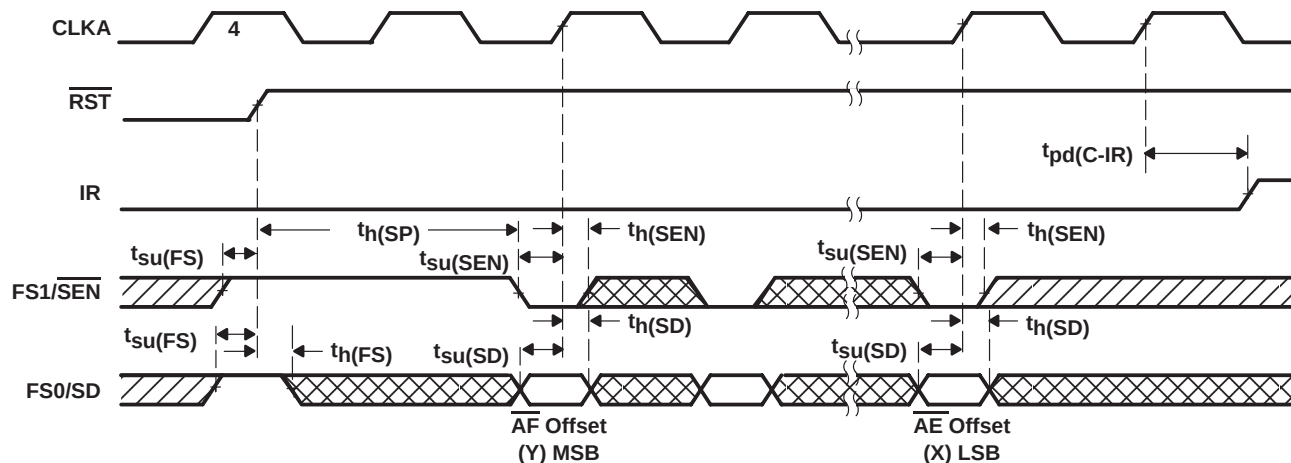
Figure 3. Programming the \overline{\text{AF}} Flag and \overline{\text{AE}} Flag Offset Values Serially
