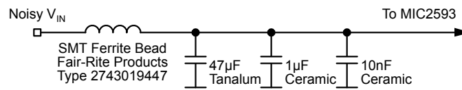
Figure 14. Filter Circuit for Noisy Supplies ( +3.3\text{V} and/or -12\text{V} )
