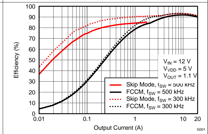
Figure 12. Efficiency vs. Output Current
