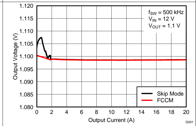
Figure 10. Output Voltage vs. Output Current
