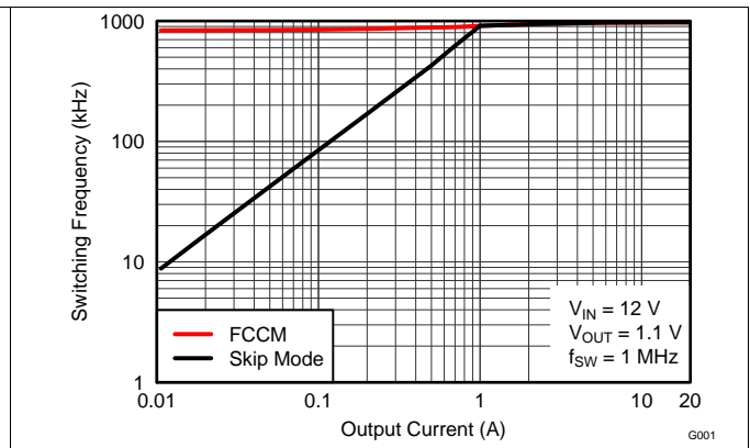
Figure 8. Switching Frequency vs. Output Current
