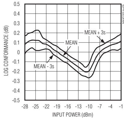
LOG CONFORMANCE WITH 1dB STEP PCS BAND
