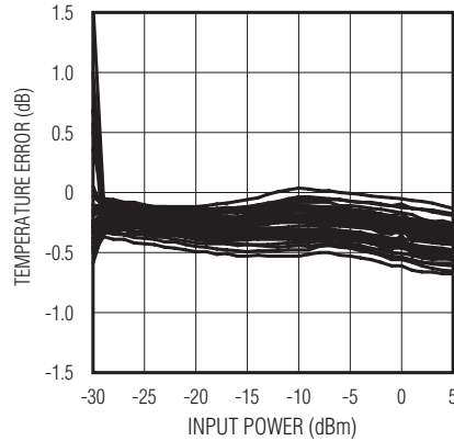
47-UNIT CELLULAR ROOM-HOT TEMPERATURE ERROR
