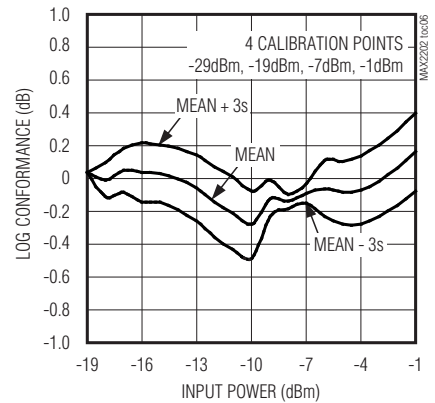
LOG CONFORMANCE WITH 10dB STEP CELLULAR BAND
