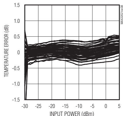
47-UNIT CELLULAR ROOM-COLD TEMPERATURE ERROR
