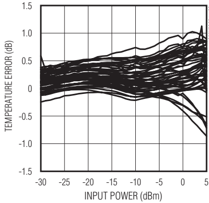
47-UNIT PCS ROOM-COLD TEMPERATURE ERROR
