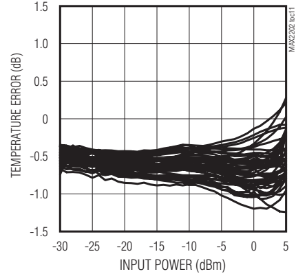
47-UNIT PCS ROOM-HOT TEMPERATURE ERROR
