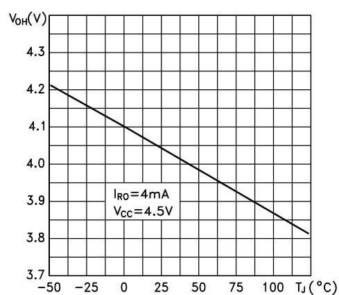
Figure 15: Receiver high level output voltage vs. temperature
