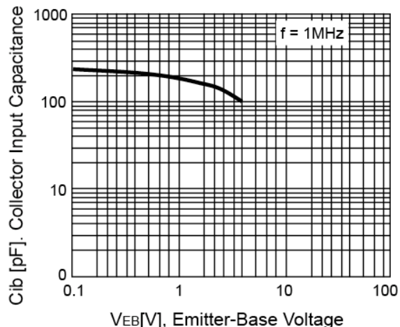
Figure 6. Collector Input Capacitance vs. V_{EB}
