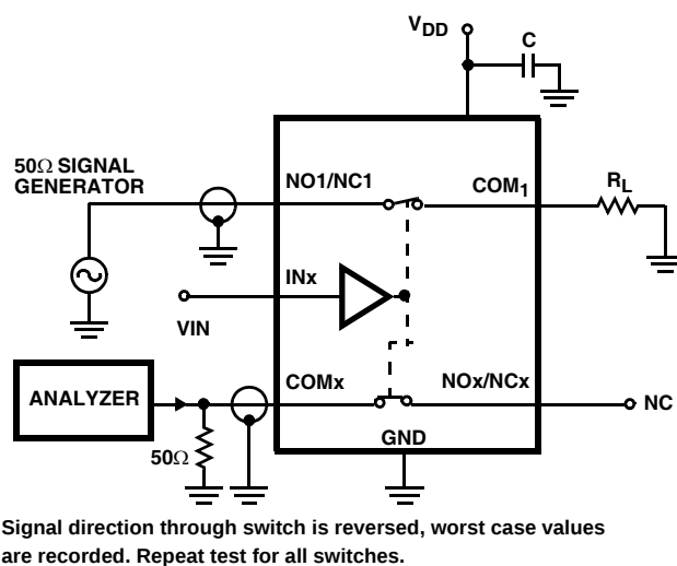
FIGURE 4. CROSSTALK TEST CIRCUIT
