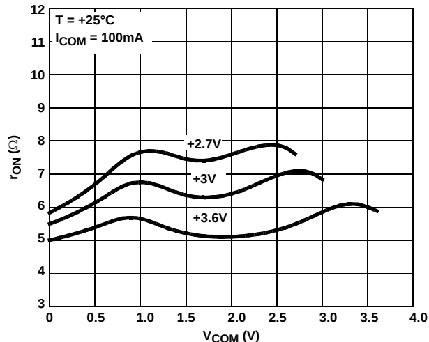
FIGURE 14. ON-RESISTANCE vs SWITCH VOLTAGE; COM1B AND COM4B
