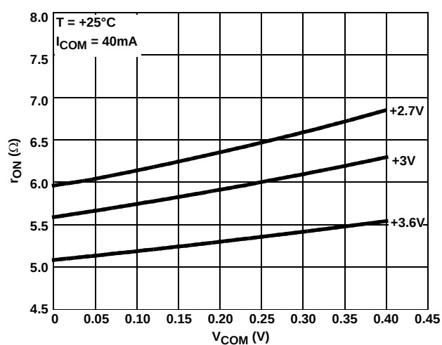
FIGURE 8. ON-RESISTANCE vs SWITCH VOLTAGE; COM2, COM3
