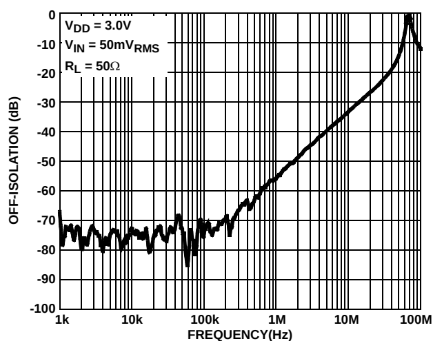
FIGURE 18. OFF-ISOLATION; COM1A AND COM4A
