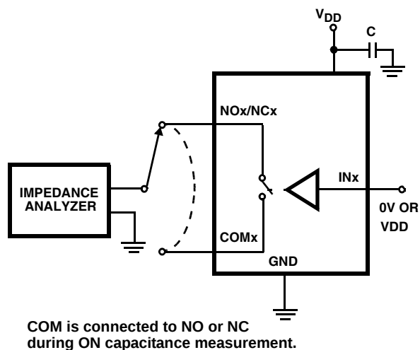
FIGURE 3. CAPACITANCE TEST CIRCUIT
