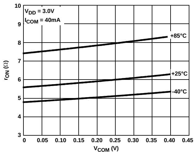
FIGURE 7. ON-RESISTANCE vs SWITCH VOLTAGE; COM2x AND COM3x
