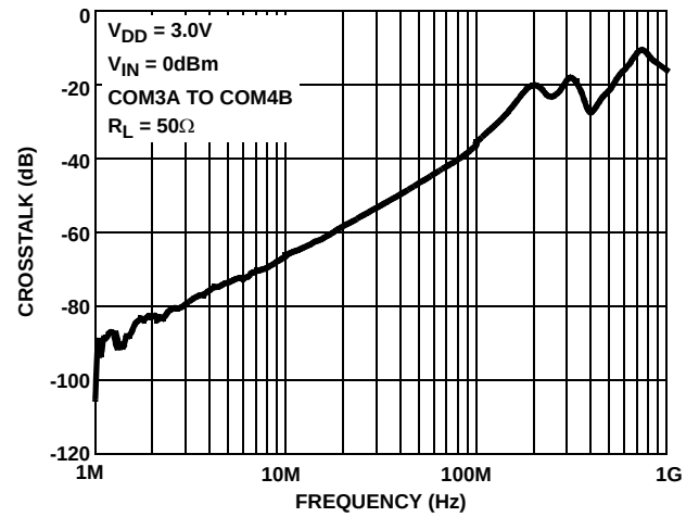
FIGURE 22. CROSSTALK
