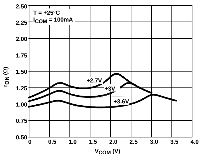
FIGURE 12. ON-RESISTANCE vs SWITCH VOLTAGE; COM1A AND COM4A
