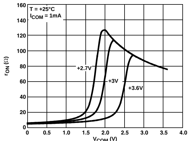
FIGURE 10. ON-RESISTANCE vs SWITCH VOLTAGE; COM2x AND COM3x
