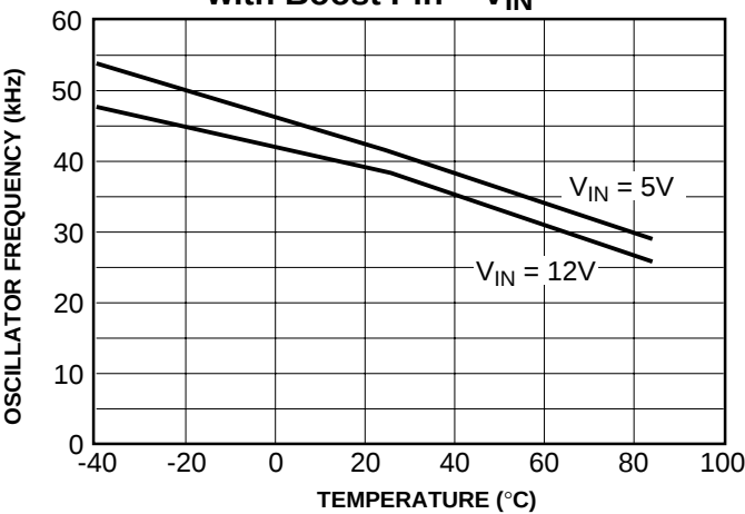
Unloaded Osc Freq vs. Temperature with Boost Pin = V_{IN}
