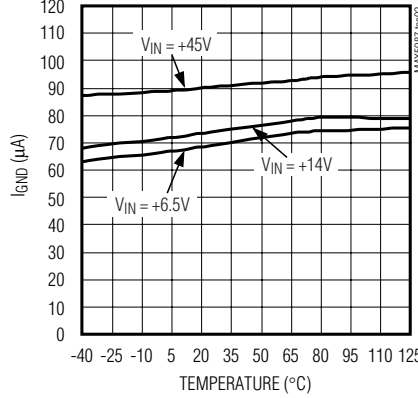
GROUND CURRENT vs. TEMPERATURE (PULSED LOAD)
