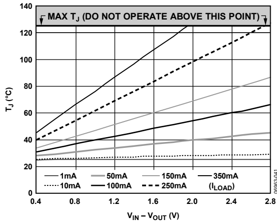
Figure 41. 100 mm 2 of PCB Copper, T_A = 25^\circ\text{C} , TSOT
