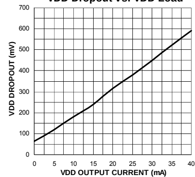
VDD Dropout vs. VDD Load
