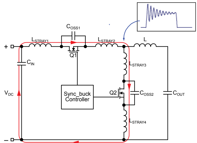
Figure 6. Output Parasitics
