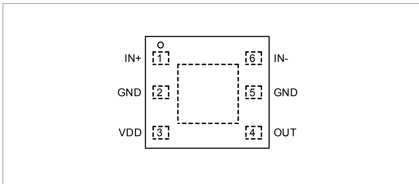
Figure 4 Pin Configuration PG-WSO6-1 (top side view)
