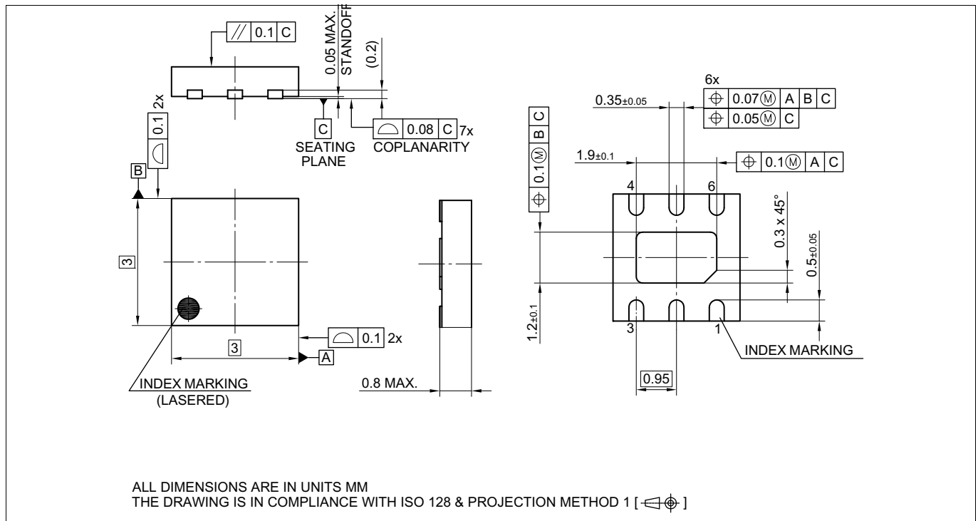
Figure 23 PG-WSN-6-1 Outline Dimensions
