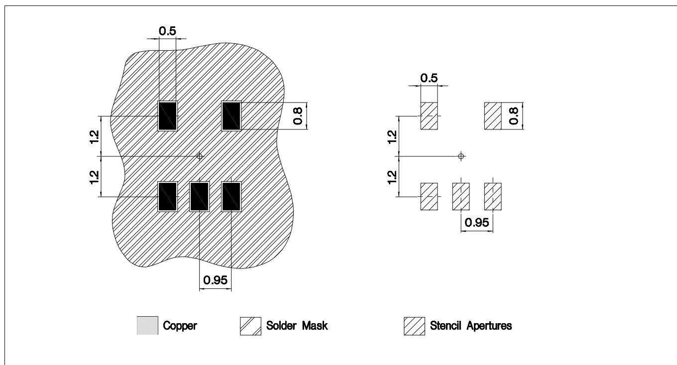
Figure 21 PG-SOT23-5-1 Footprint Dimensions
