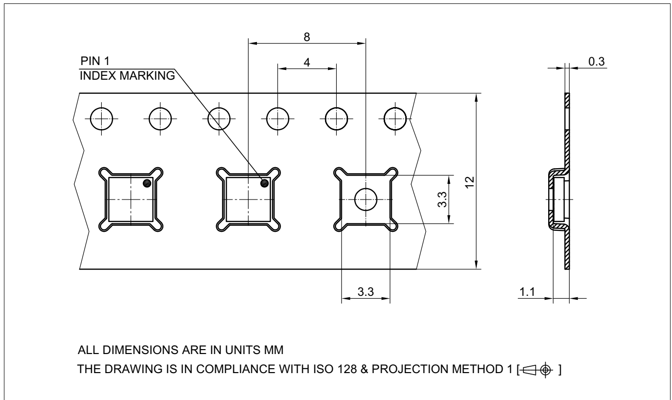
Figure 25 PG-WSO6-1 Packaging Dimensions
