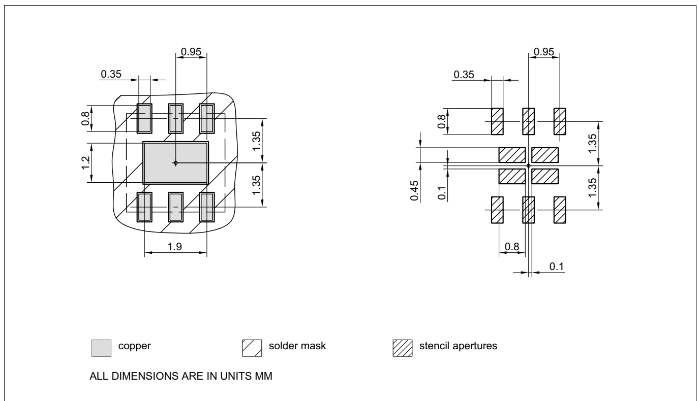
Figure 24 PG-WSN-6-1 Footprint Dimensions
