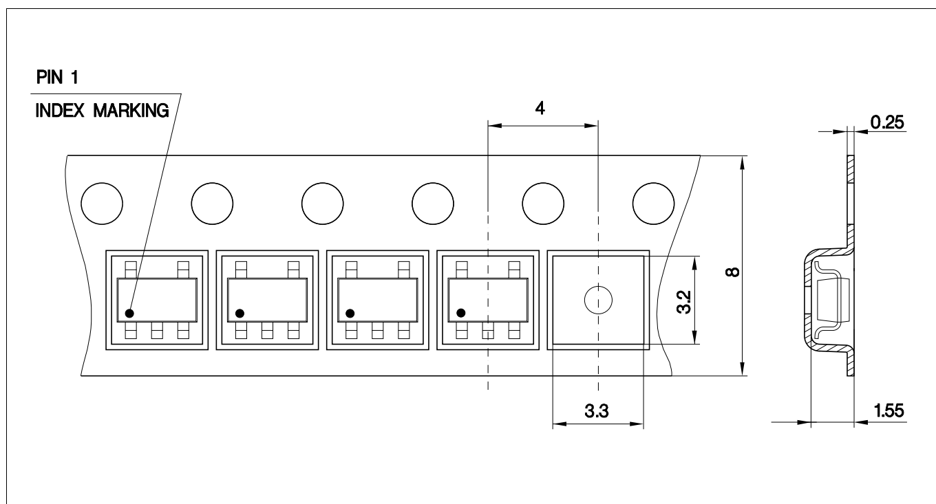
Figure 22 PG-SOT23-5-1 Packaging Dimensions
