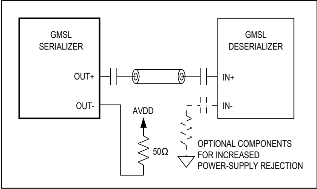
Figure 15. Coax Connection
