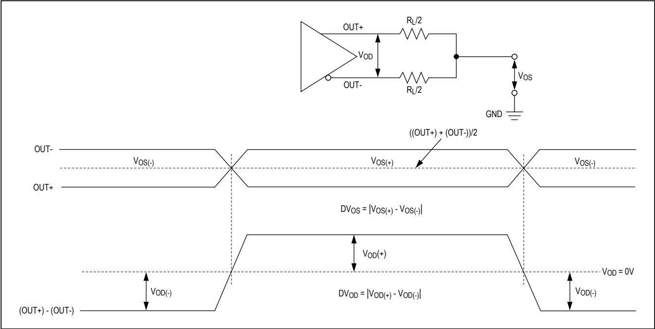
Figure 1. Serial-Output Parameters
