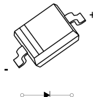
SOD-323
