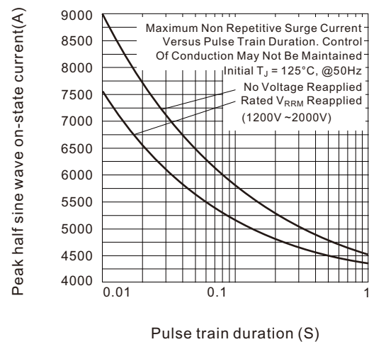
Fig.10 Maximum non-repetitive surge current single and double side cooled
