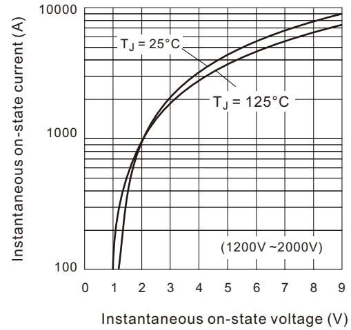
Fig.14 On-state voltage drop characteristics
