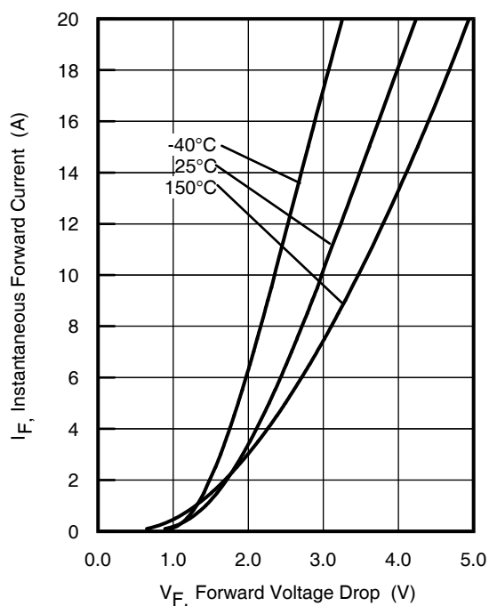
Fig 1. Typical Forward Characteristic
