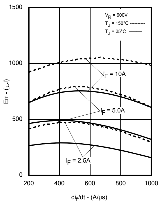
Fig 5. Typical Err vs. di/dt
