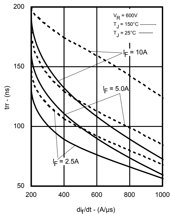
Fig 2. Typical t_{rr} vs. di/dt
