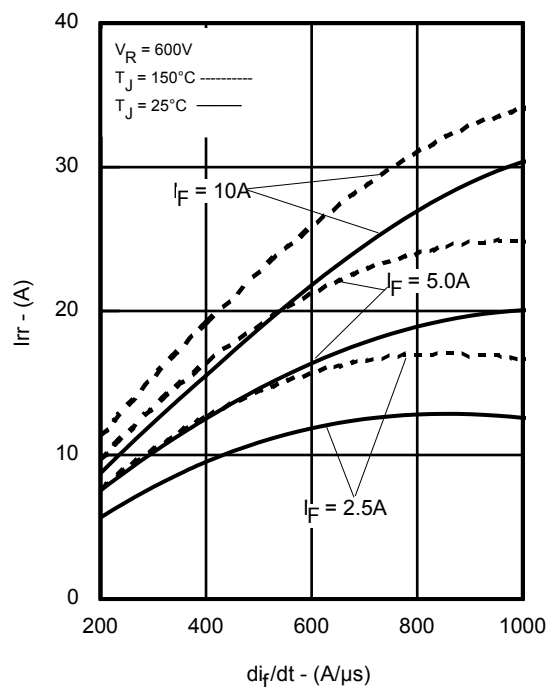
Fig 4. Typical I_{rr} vs. di/dt
